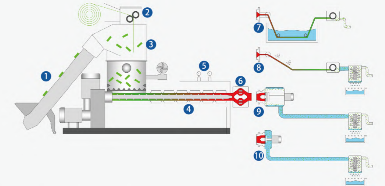
1 Belt conveyor
